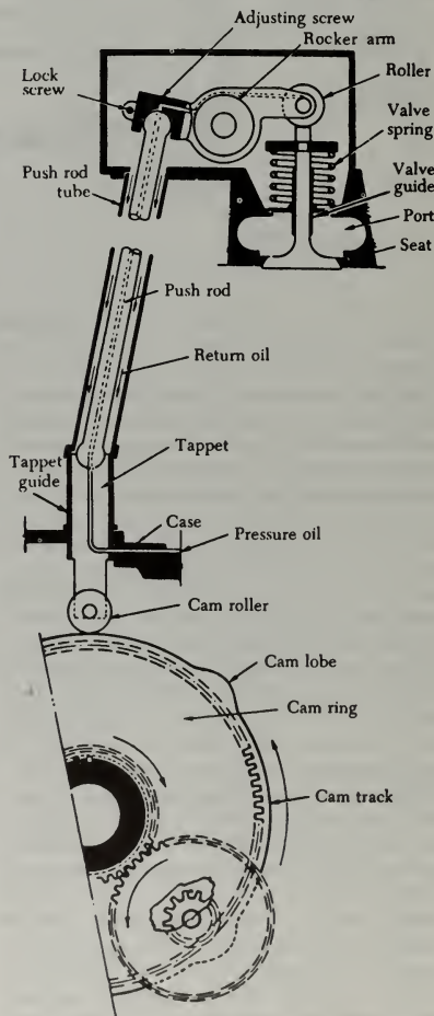
FIGURE 1-18. Valve-operating mechanism (radial engine).
